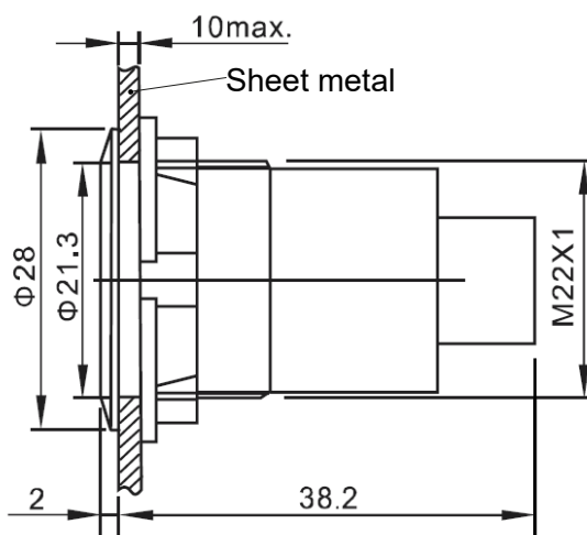
Lateral view
