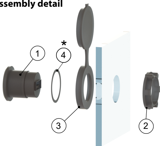
Assembly detail
